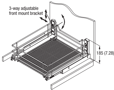
▶ With frameless slide and one spacer
