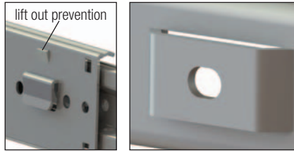
Mounting Lance with security screw slot
